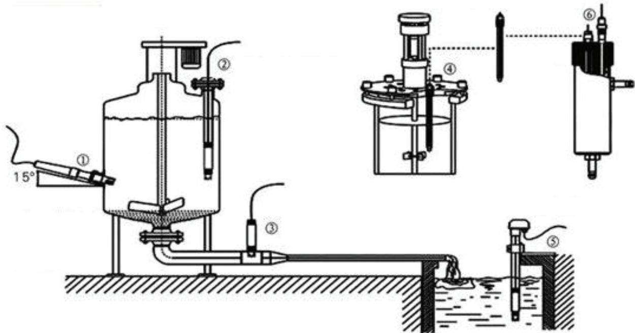
Schematic diagram of common installation method
